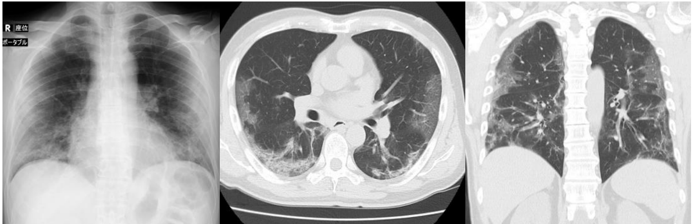
Fig.1 COVID-19肺炎
